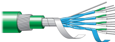
XLPE / ICAT / LS0H / GSWA / LS0H
