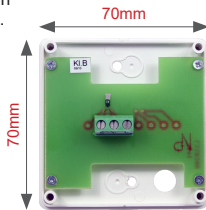
Inside view showing cable terminal and mounting holes
